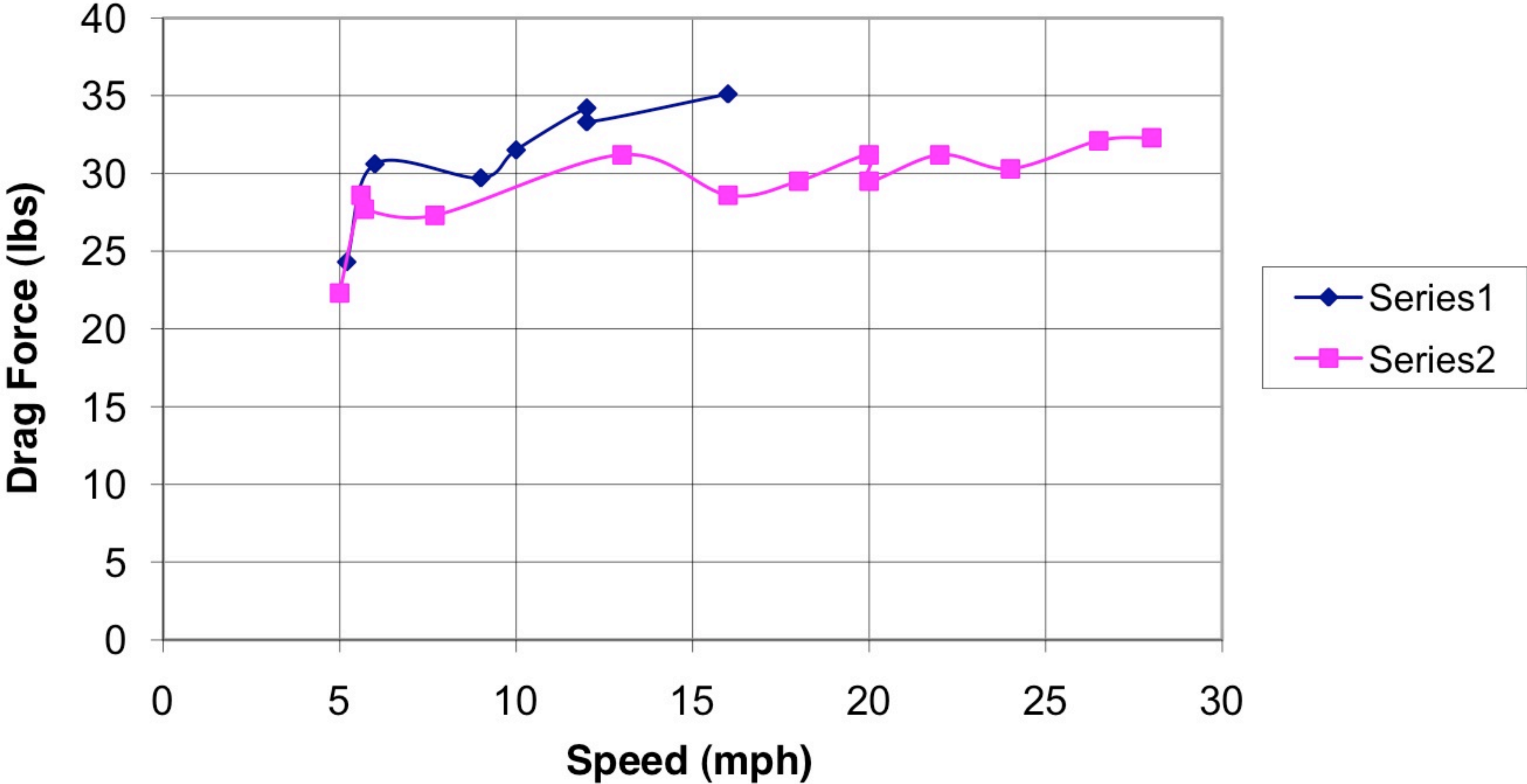
Fig. 7 Effect of Step Design on 66cm Wide Board
