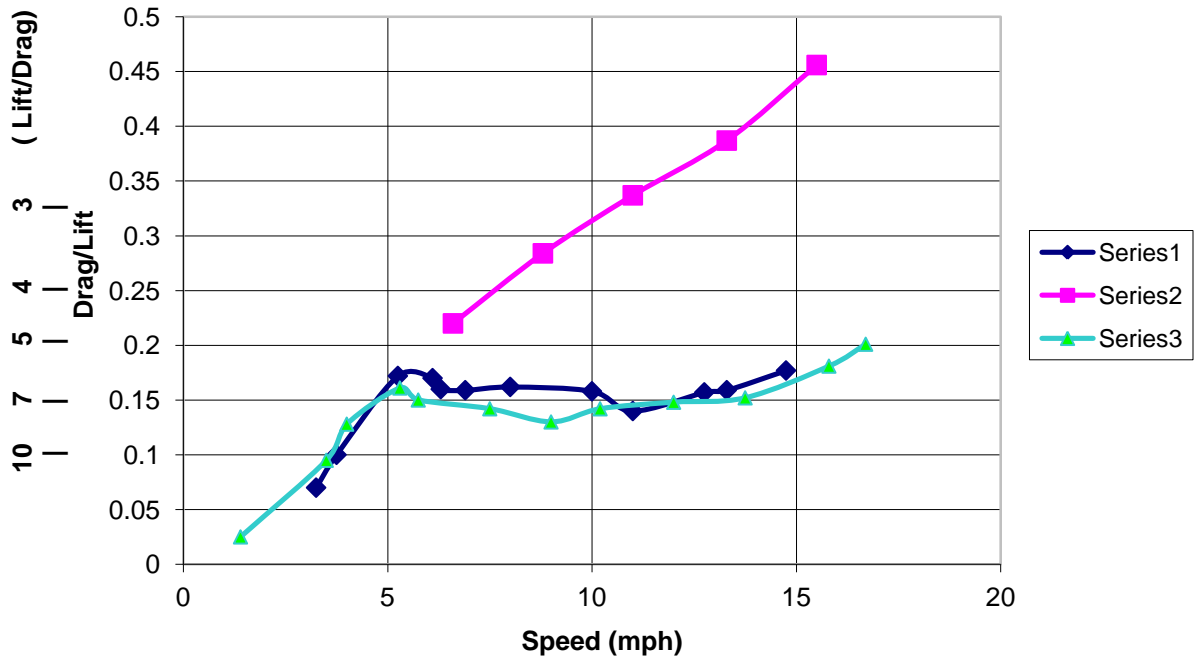
Fig. 8 Yacht Model Drag
